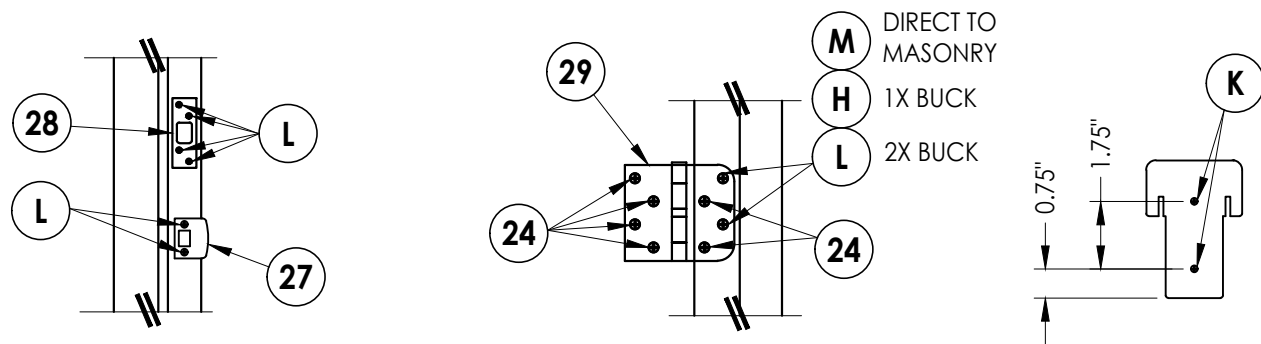
LATCH AND DEADBOLT Details
